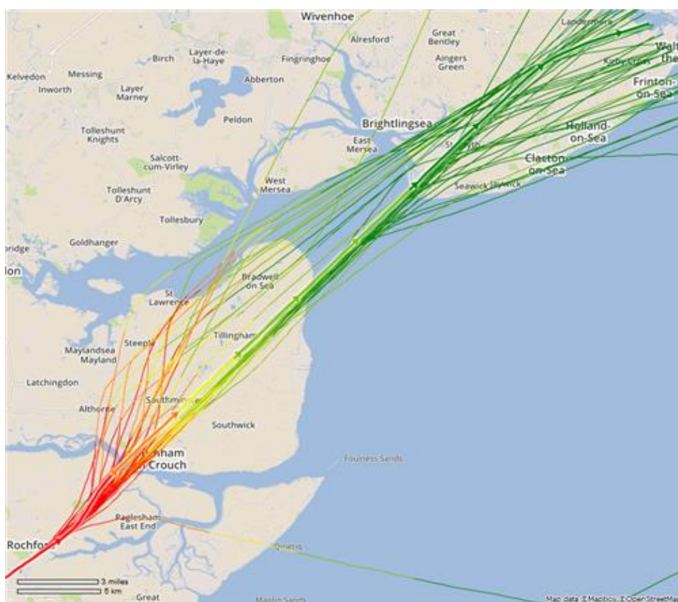
Figure E5: Colour coded climb profile of departing flights Summer 2015
