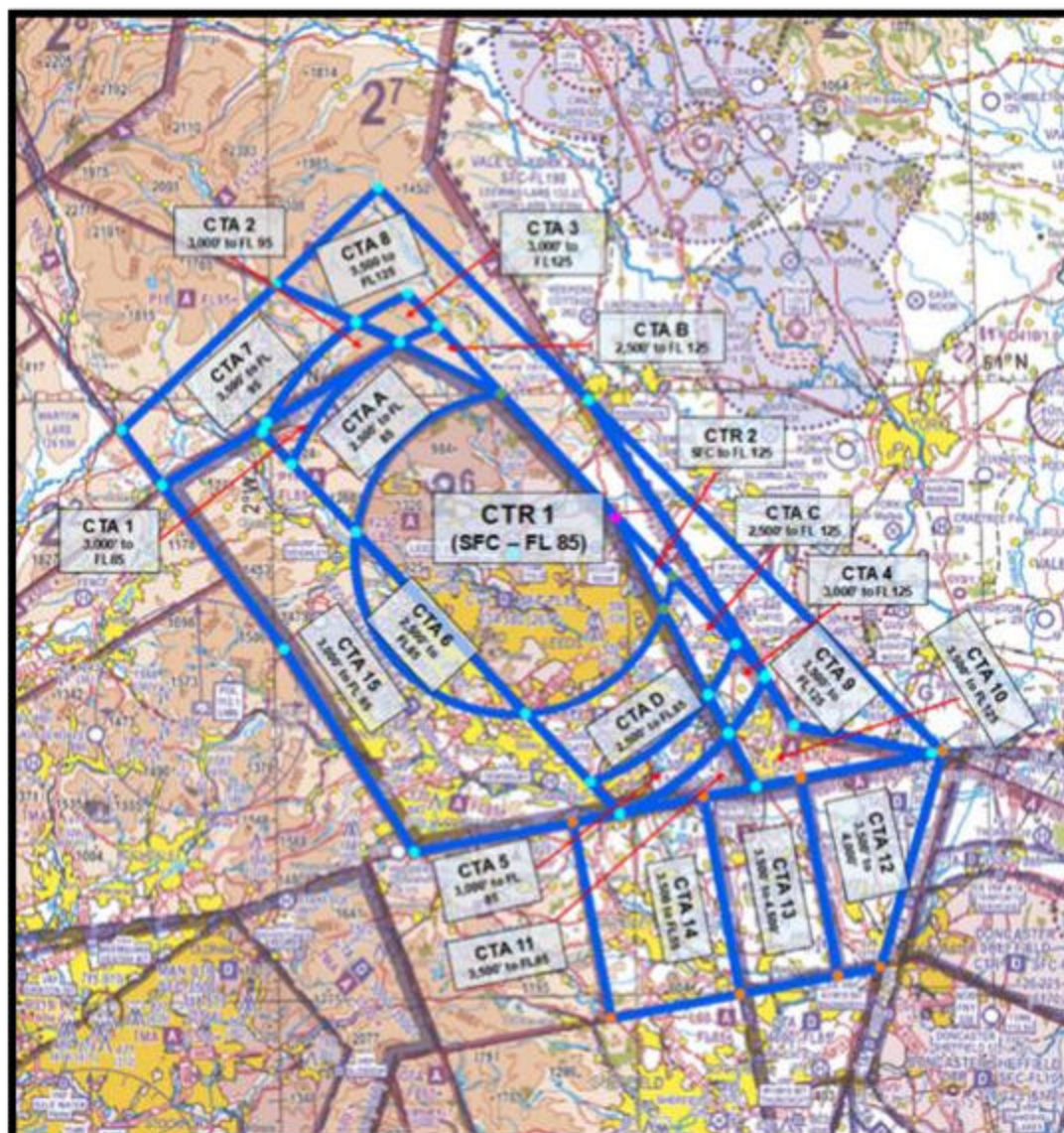
Figure 7 – Post Consultation Airspace Design
