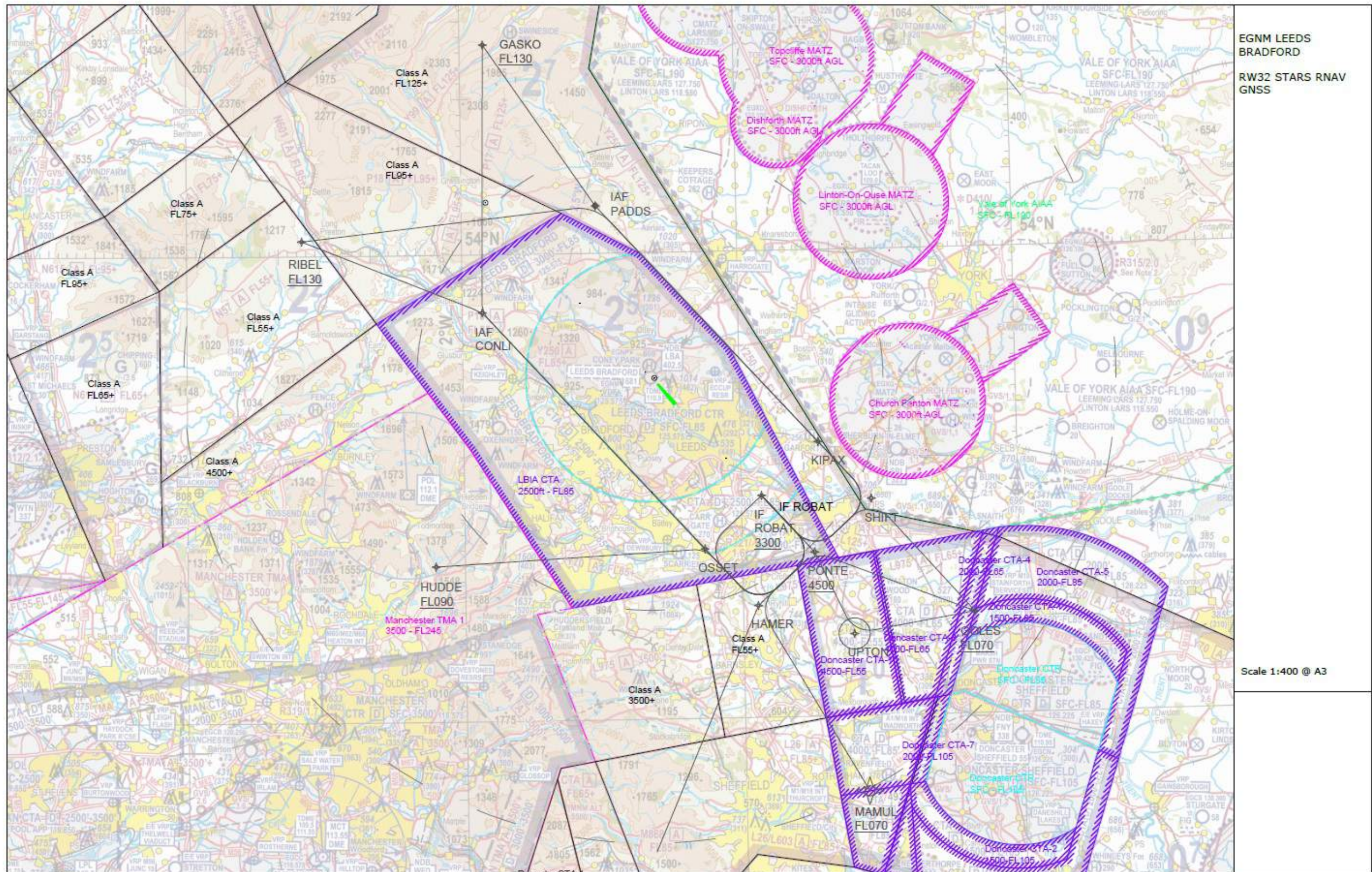
Figure 7. Draft Arrival Routes to Runway 32
