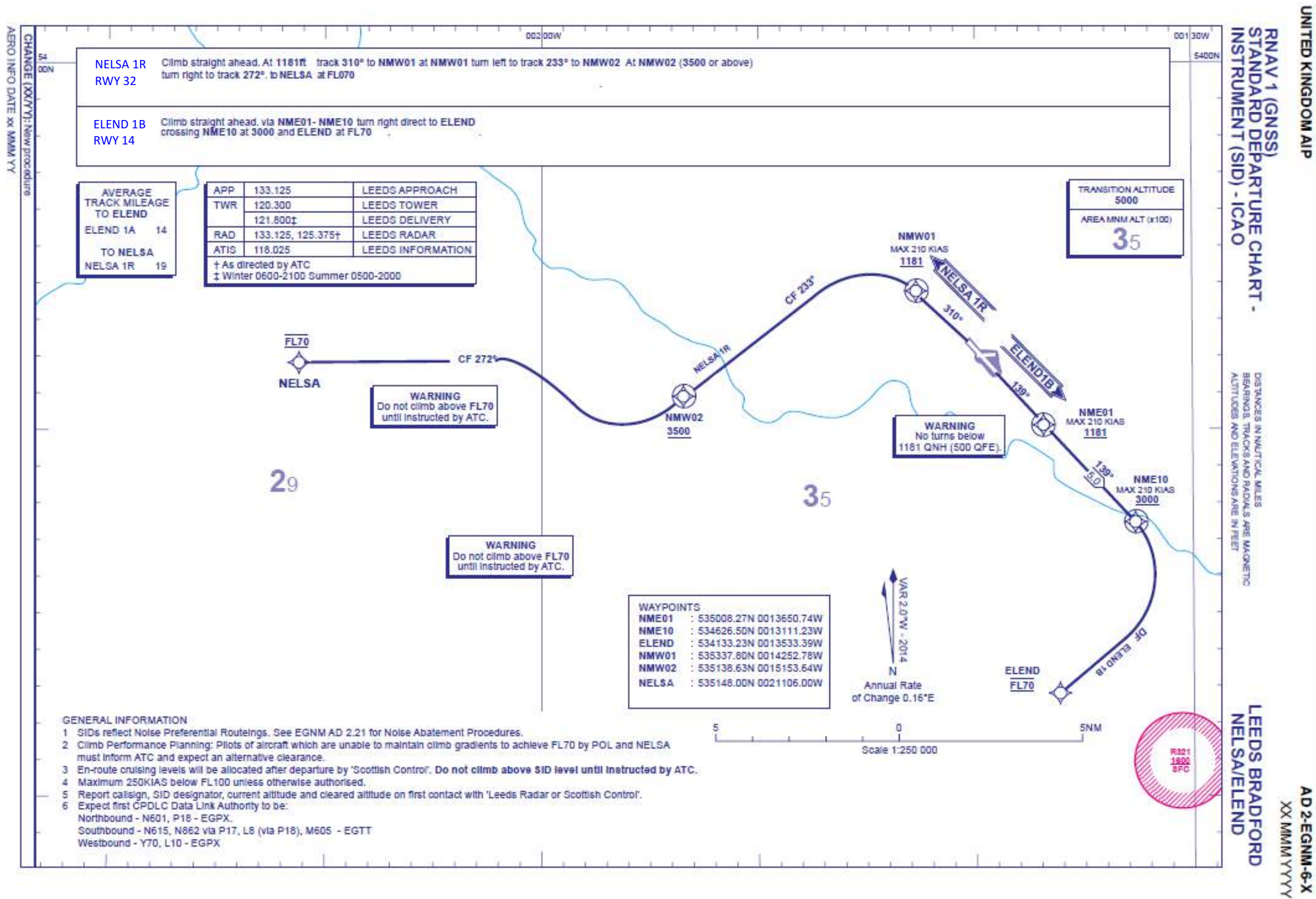
Figure 5. Draft GNSS Standard Instrument Departures – NELSA/ELEND
