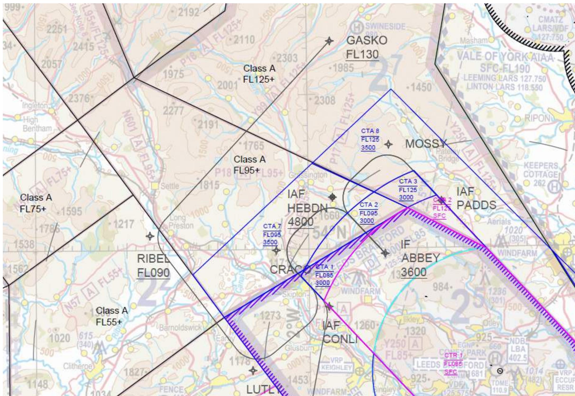
Figure 8. Draft Arrival Routes from the North to Runway 14
