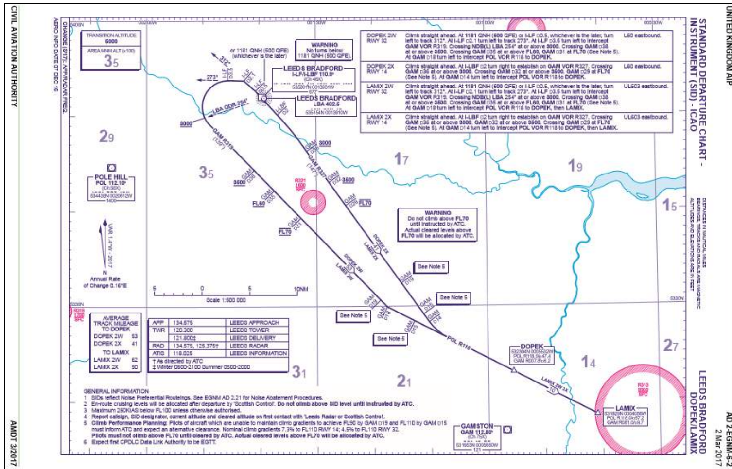
Figure 1. Current Standard Instrument Departures – DOPEK/LAMIX (Available at http://www.ead.eurocontrol.int/eadbasic/pamslight-0EA5010DC20CC86C50175510792BC9F9/7FE5QZZF3FXUS/EN/Charts/AD/AIRAC/EG_AD_2_EGNM_6-2_en_2017-03-02.pdf )
